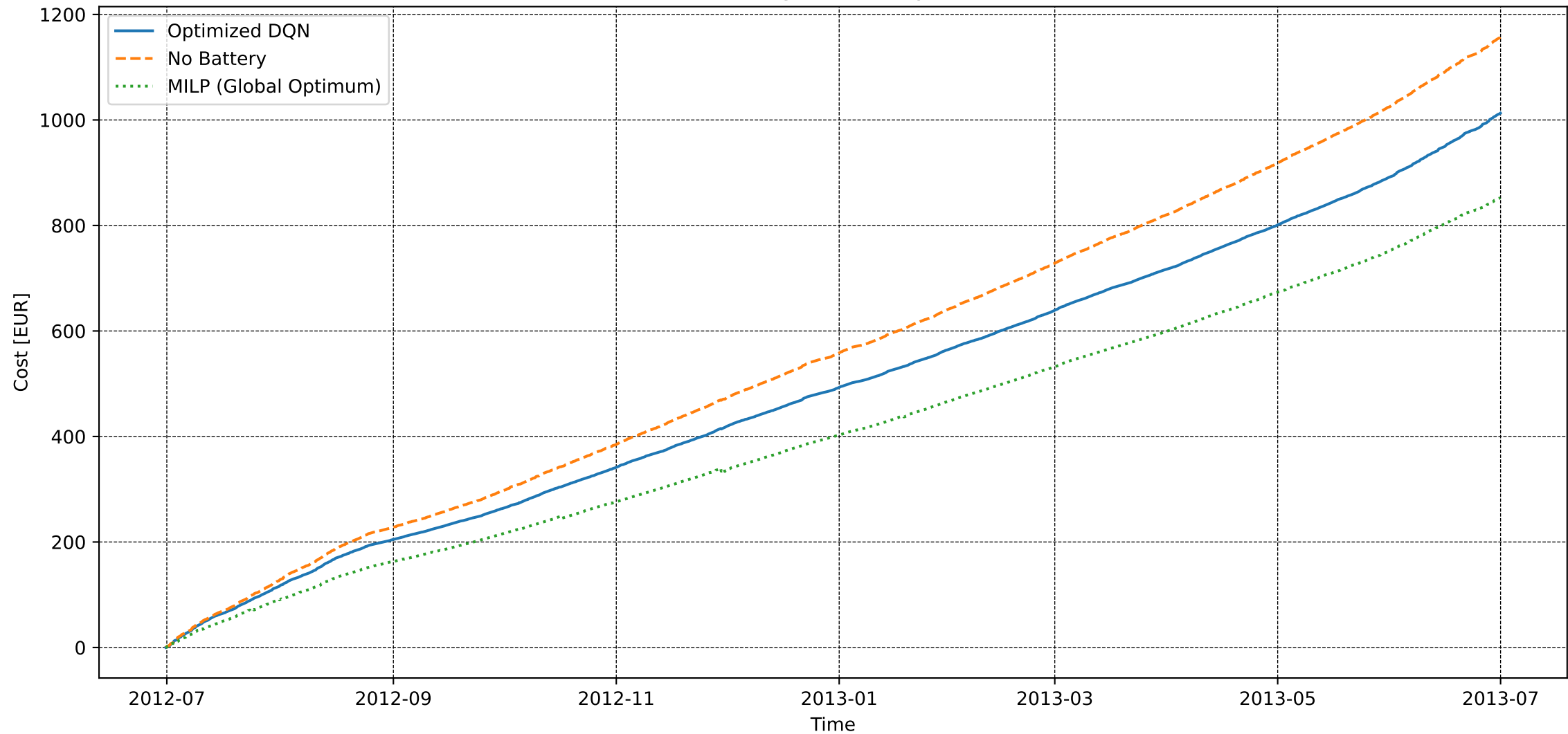
User 142 - Basic Training - Electricity Cost [DQN vs MILP]
